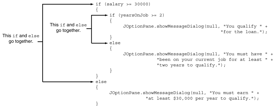
Figure 3-14 Alignment of if and else clauses
